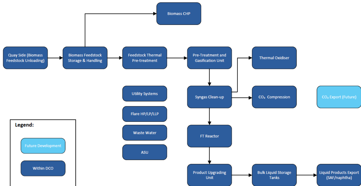
Figure 2.1: SAF Production Process
